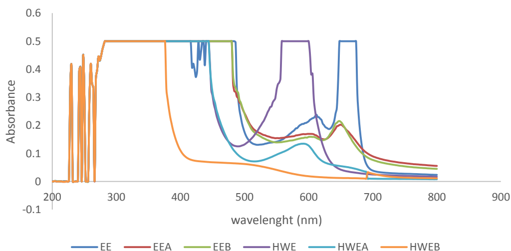
Fig. 2. UV/visible absorption spectra of ethanol and hot water extracts of Declipitarea verticilata leaves in different media
