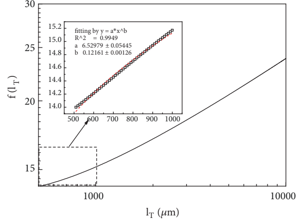
FIGURE 3: The effect of the thermal length on the scaling law of formula (5). The inset presents the local region with power law fitting. The corresponding parameters are \lambda_2 \approx 350V^{-0.6} with V=50 \mu\text{m/s} , a=0.1 , and n=2 .
