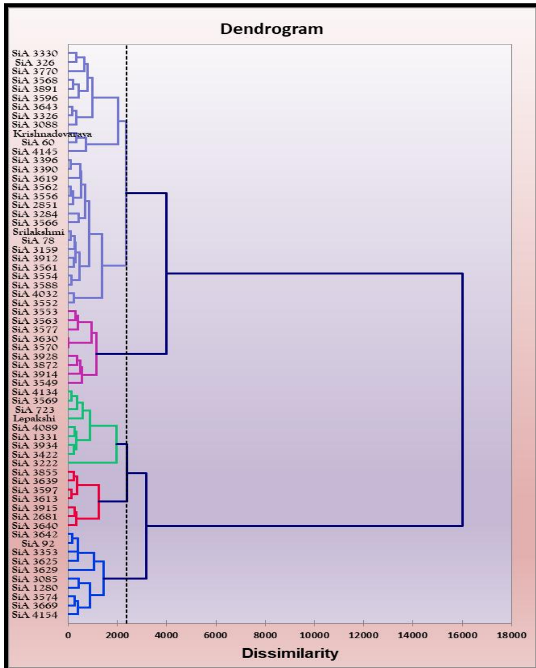
Fig. 3. Dendrogram showing relationship in five clusters based on Euclidian 2 distance in 64 genotypes of foxtail millet ( Setaria italica (L.) Beauv.)
