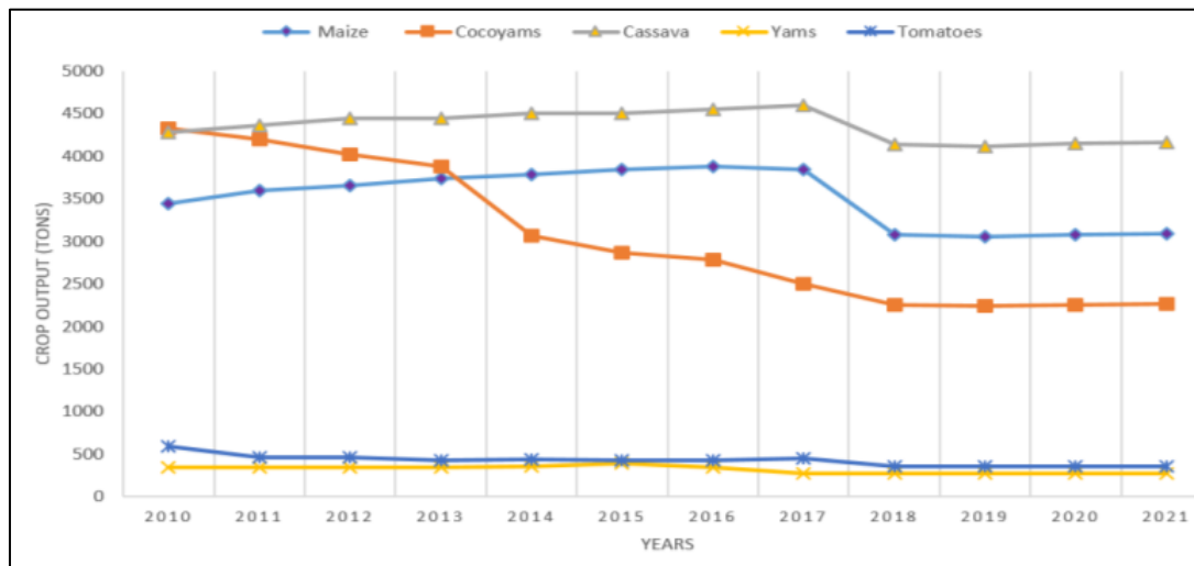
Fig. 9. Decline in crop output in Santa between 2010 and 2021
