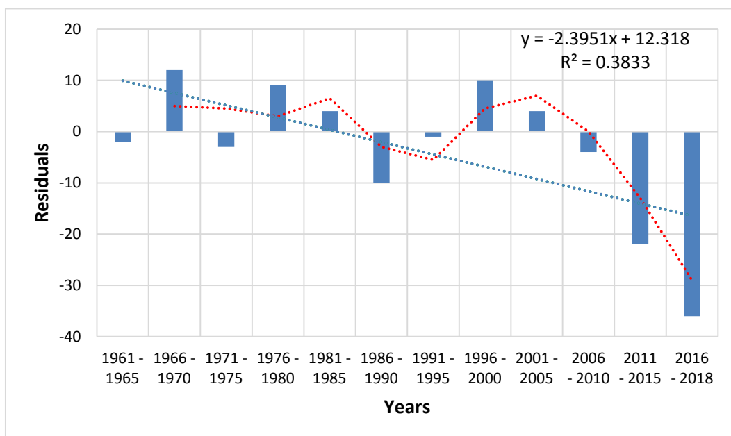
Fig. 7. Variations in rainy days in the Western Highlands between 1961 and 2018
