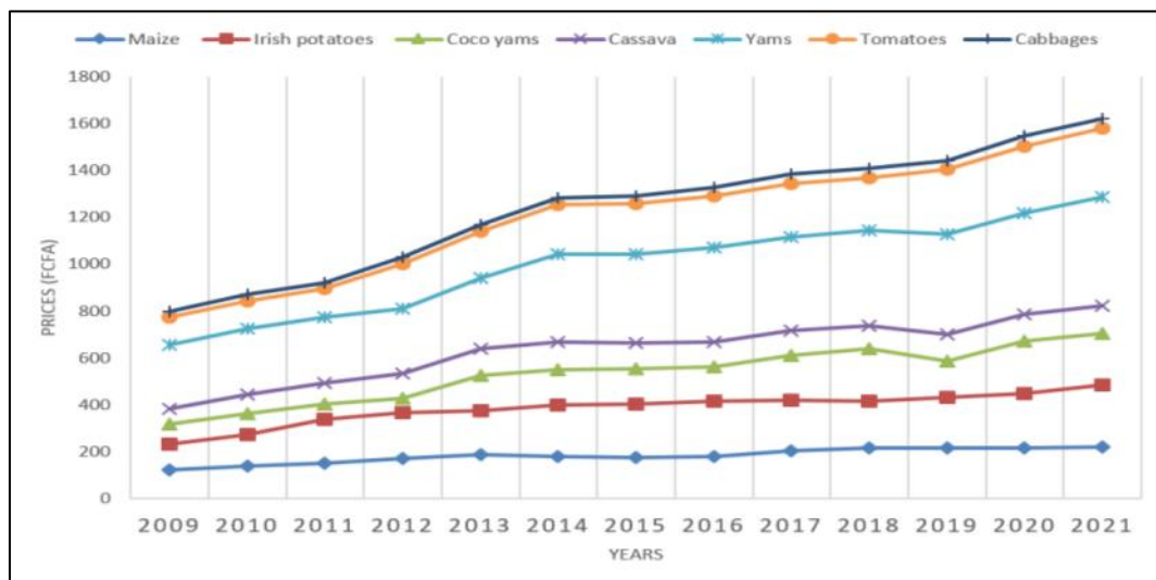
Fig. 10. Evolution in the prices of selected crops in Santa (2009 to 2021)
