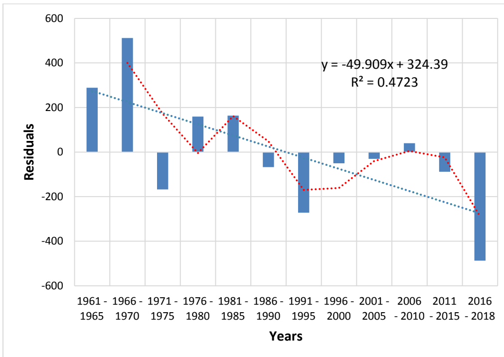
Fig. 6. Variations in rainfall in the Western Highlands between 1961 and 2018
