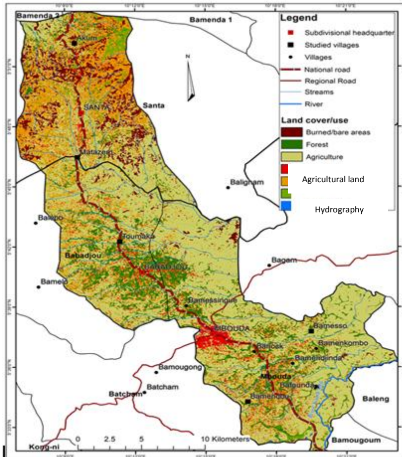
Fig. 3. Land cover/use for the southern part of the Western Highlands in 2002
