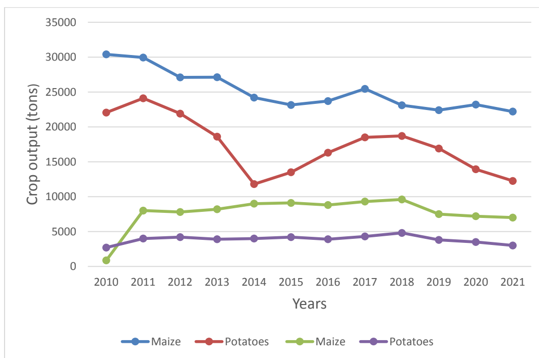
Fig. 8. Declining trends in maize and Irish potatoes output in Mbouda and Babadjou
