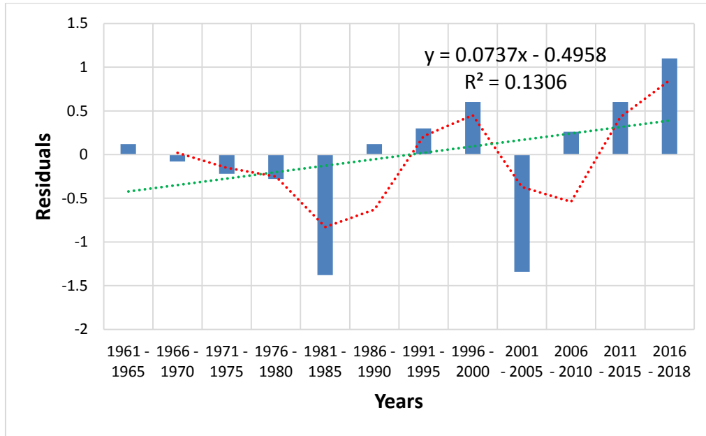
Fig. 5. Variations in temperature in the Western Highlands between 1961 and 2018
