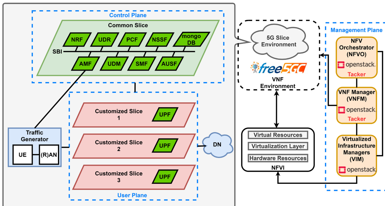
Figure 4. Our proposed 5G slice architecture.
