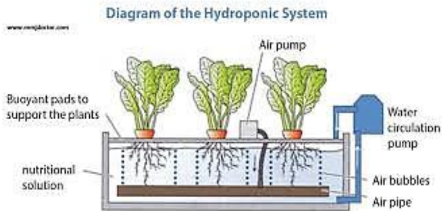
Fig. 2. Diagram of the Hydroponic System
