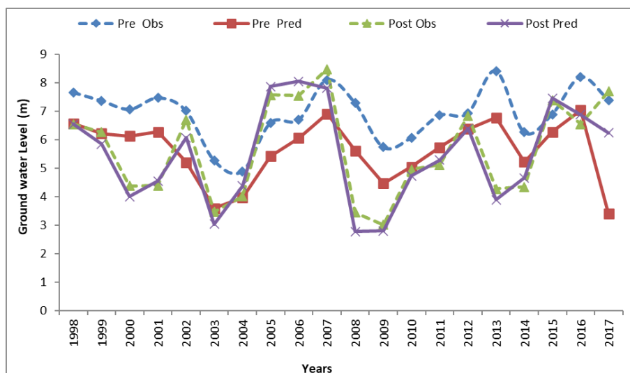
Fig. 1. Observation and prediction of pre and post monsoon ground water level at different locations
