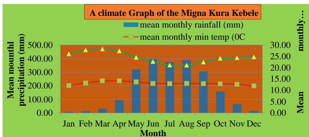
Fig. 2. Mean monthly rainfall, max and min temperatures of the study area (2006 – 2018).
