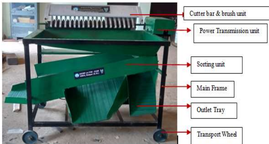
Fig. 1. Developed onion stem and root cutter cum sorting machine
