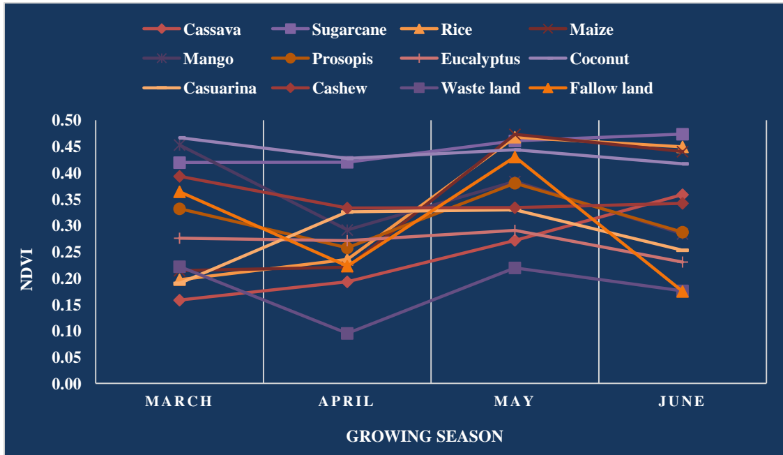
Fig. 6. NDVI trends of different crops from March - June
