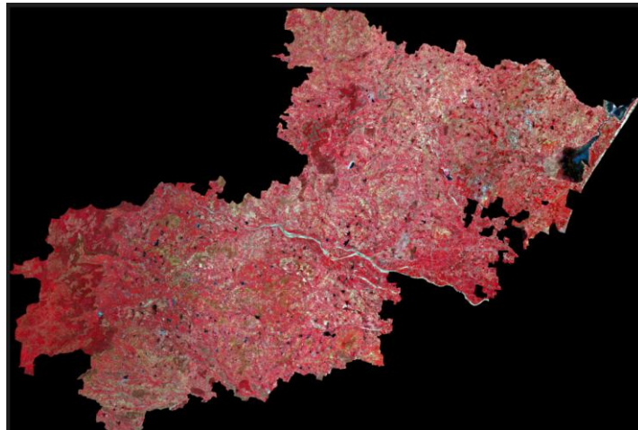
Fig. 3. False colour composite image of the study area
