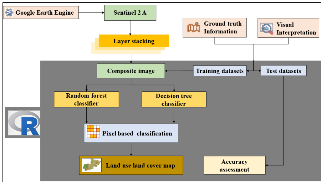
Fig. 2. Methodology for land use land cover mapping
