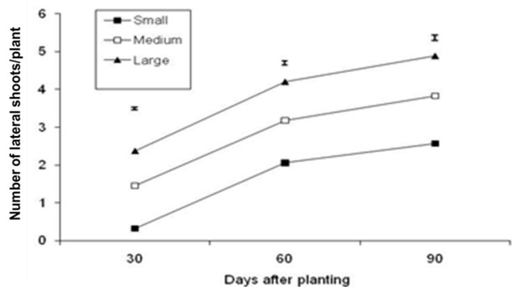
Fig. 2. Lateral shoot production in tuberose as influenced by bulb sizes at different plant age. Vertical bars represent LSD (0.05)
