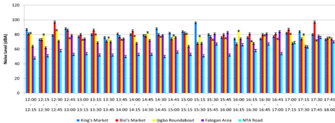
Fig. 6. Noise generation level (dBA) in market areas
