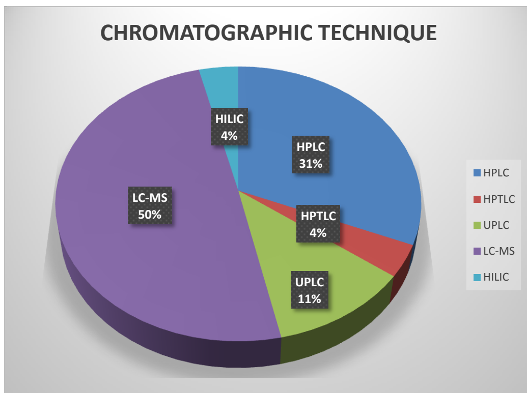
Fig. 8. Different Chromatographic Technique used for Impurity and Forced degradation profiling of Antidiabetic drugs
