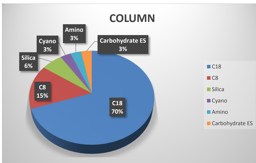
Fig. 4. Different column used for of Impurity and Forced degradation profiling of Antidiabetic drugs
