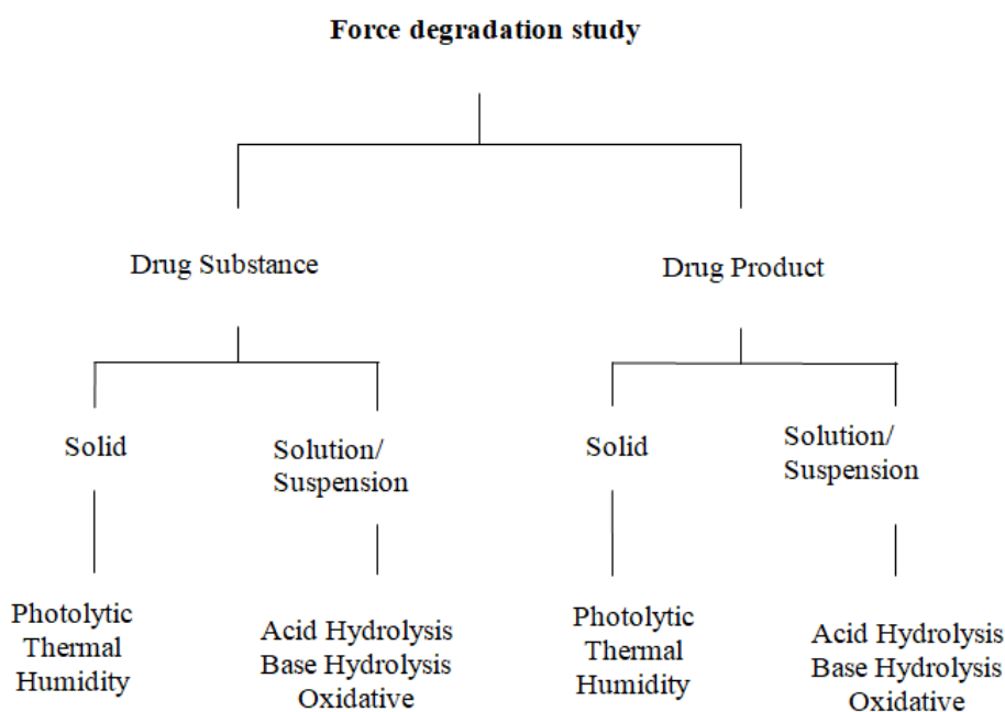
Fig. 3. Force degradation study
