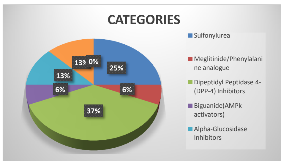
Fig. 7. Categories of Antidiabetic drugs on which impurity profiling and forced degradation are studied
