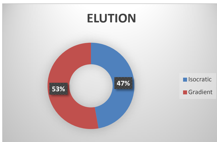
Fig. 5. Types of Elution performed in analysis for Impurity degradation profiling of Antidiabetic drugs
