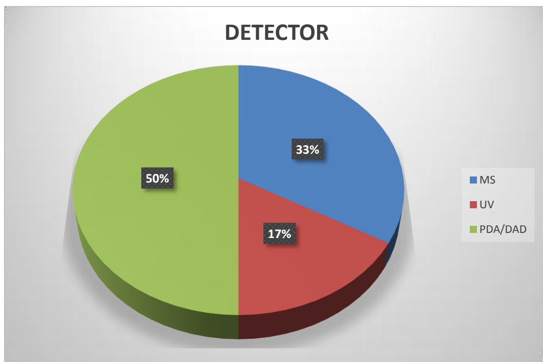
Fig. 9. Different detectors used for Impurity and Forced degradation profiling of Antidiabetic drugs
