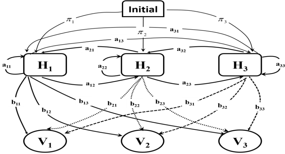
Fig. 1. Schematic diagram of HMM
