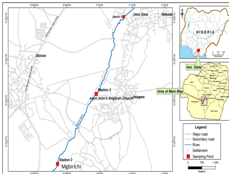
Fig. 1. Map of Otamiri River showing the sampling stations (Sources: Cartographic Unit,, University of Ibadan, 2019)
