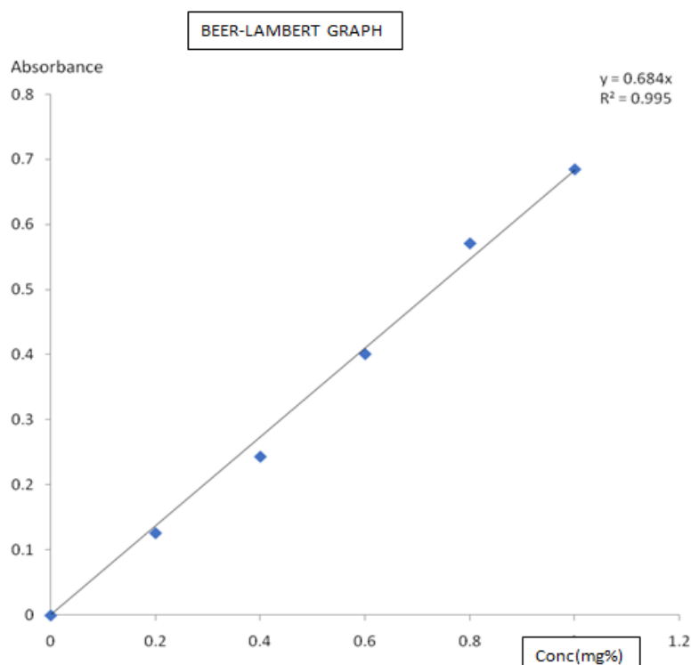
Fig. 1. Beer's plot of acetaminophen in 0.1N hydrochloric acid at 290nm and 37±1
