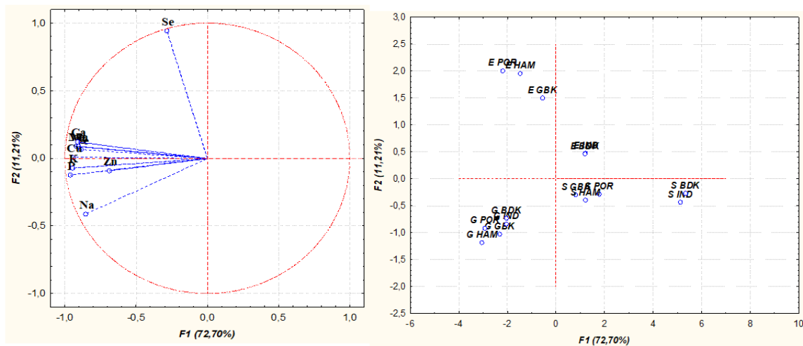
Fig. 1. Projection of essential minerals (a) and regions (b) in the factorial plane F.1 and F. 2 of the principal component analysis (PCA)
