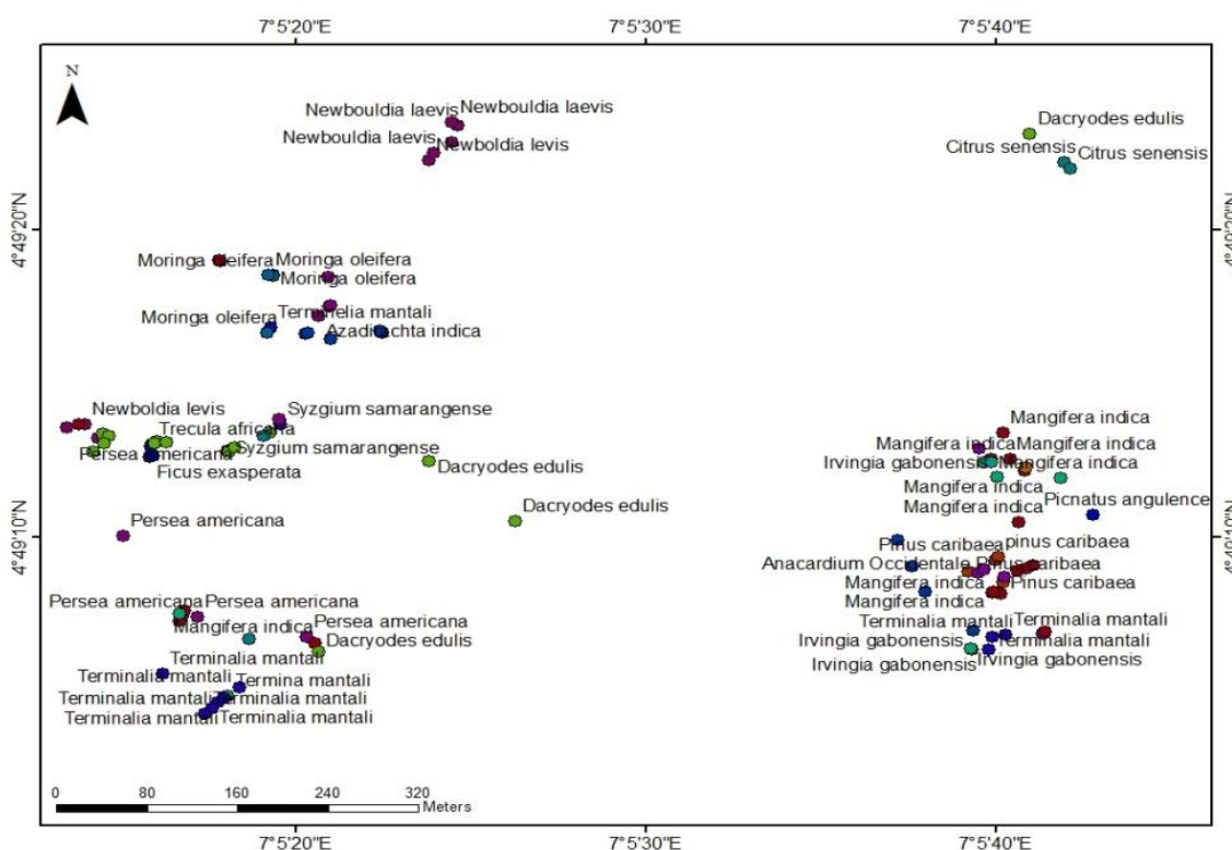
Fig. 2. Study area showing the wood trees encountered
