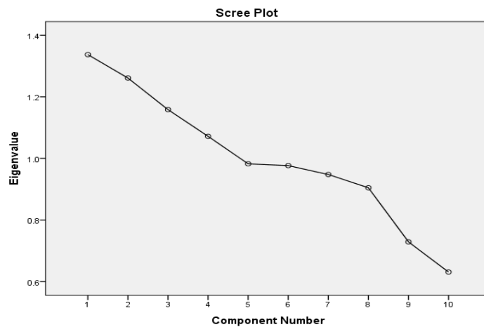
Fig. 1. Scree Plot Showing Component wise Eigen Values for Members' Social Perceptions (Source: Author, Computed)
