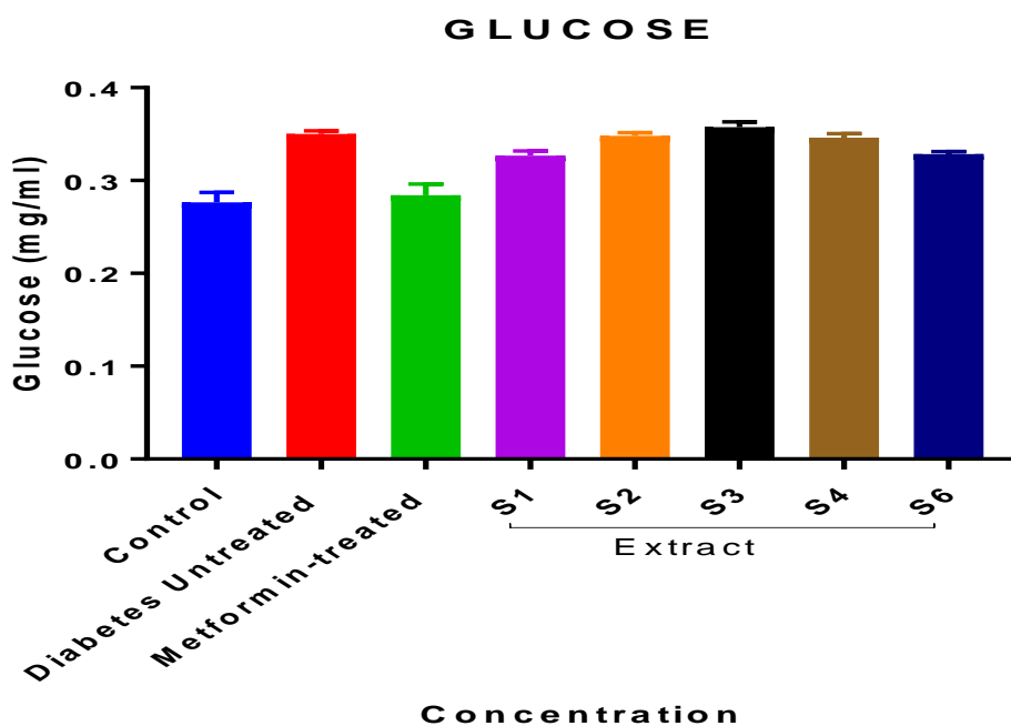
Fig. 2. The glucose content of fruit flies (diabetic) treated with Shemmeco extract
