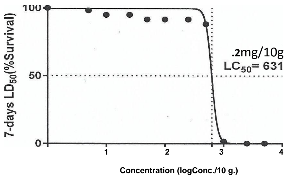
Fig. 1. LC50 curve obtained from the result of acute toxicity assay of Shemmeco extract
