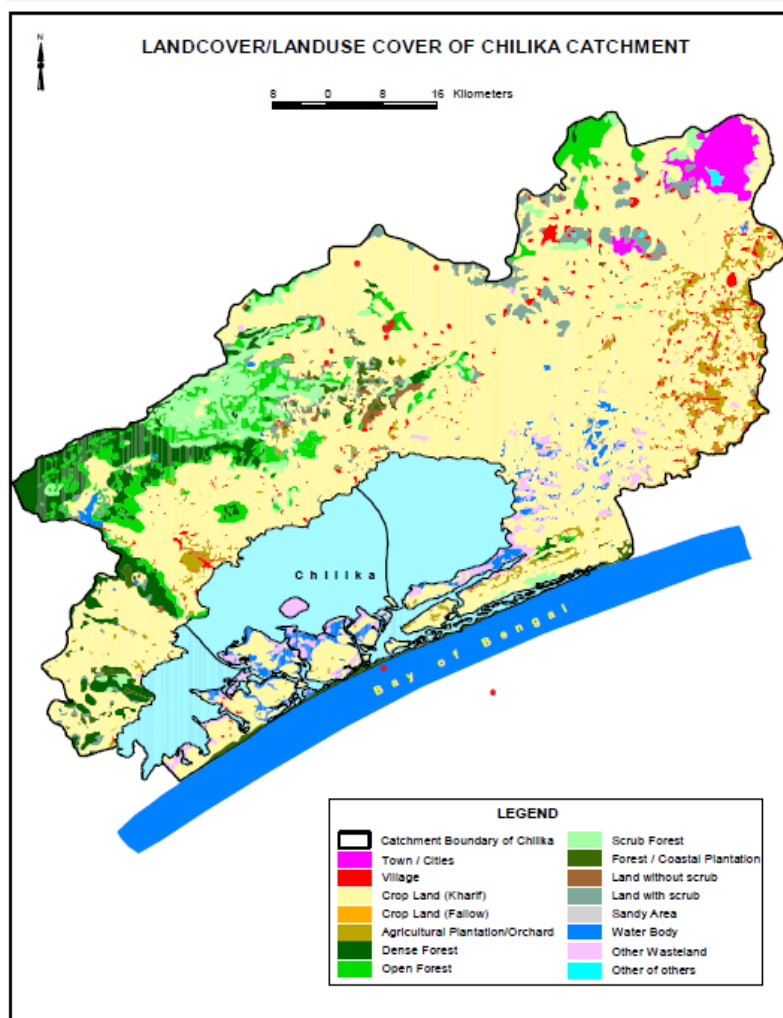
Fig. 2. Land use coverage of Chilika Catchment
