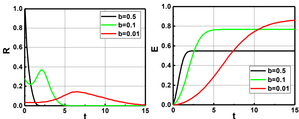
Fig. 4. The time profile of radical R(t) and efficacy, E(t) , for bl=(0.01, 0.1, 0.5) , for the case of pure type-I case (with K'=0.05 and Q=0 ); showing higher light intensity has a lower steady-state efficacy, but a faster transient value
