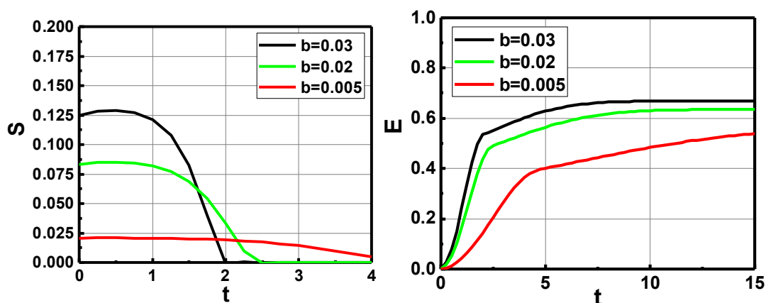
Fig. 5. The time profile of singlet oxygen S(t) and efficacy E(t) , for bl=(0.005, 0.02, 0.03) , for the case of pure type-II case (with Q=1.0 and K'R=0 ); showing the same steady-state efficacy
