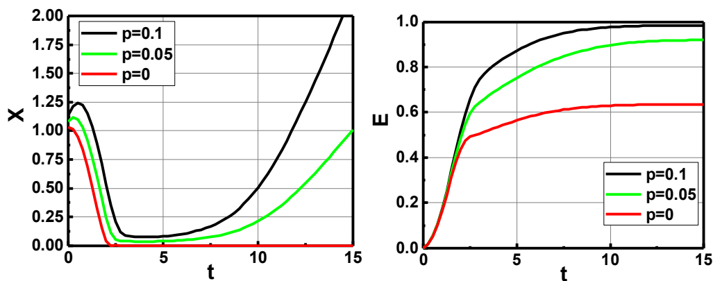
Fig. 10. The efficacy time profile of oxygen (left figure); and the associate efficacy (right figure) for various external oxygen supply with P=(0, 0.05, 0.1)
