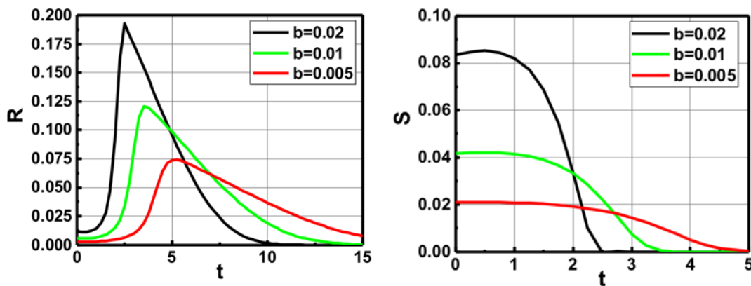
Fig. 3. The time profile of free radical R(t) and singlet oxygen S(t), with the same condition of Fig. 2
