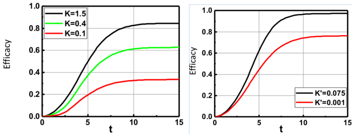
Fig. 6. The time profile of efficacy, E(t) , for various K=(0.1, 0.4, 1.5) shown by left curves; and for various K'=(0.075, 0.001) shown by right curves; for pure type-I case in the absence of oxygen (or when Q=S=0 ), with other parameters fixed as that of Fig. 4
