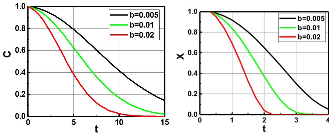
Fig. 2. The time profile of initiator, C(t), and oxygen, X(t), for various bI= (0.005, 0.01, 0.02), for cures top to low; with others parameters fixed (see text, where Q=1), where both profiles are normalized to one and time (t) is in minutes
