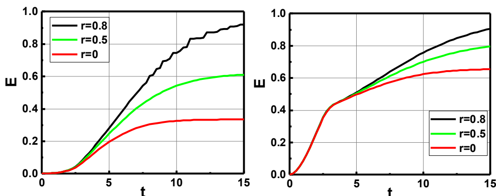
Fig. 11. The efficacy time profile of initiator C(t) , radical R(t) and efficacy E(t) , for various Re=(0, 0.5, 0.8) , with K=0.1 , K'=0.01 , b=0.02 , Q'=10 , P=0 ; and for pure type-I case (with Q=0 , left figure ); and for mixed type-I and type-II (with Q=1.0 , right figure)
