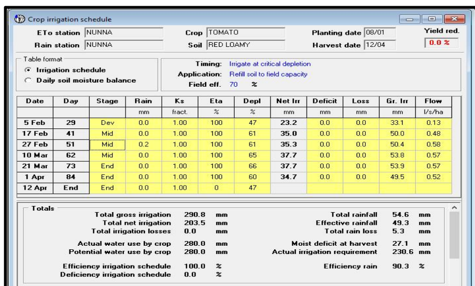
Plate 4. Irrigation scheduling in CROPWAT 8.0
