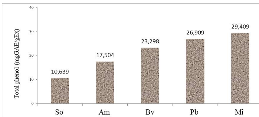
Fig. 2. Total phenol content of hydroethanolic plant extract
