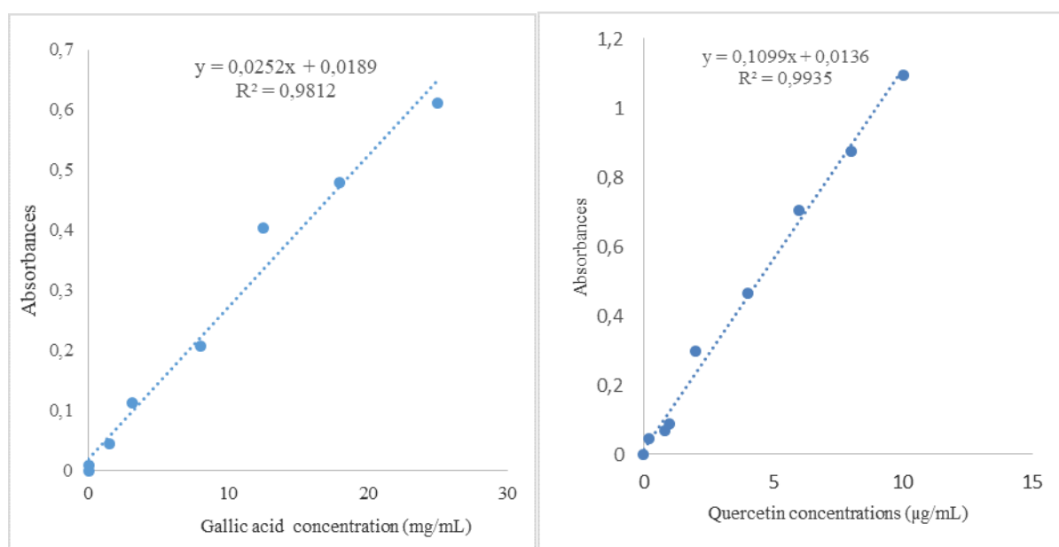
Fig. 1. Calibration curves for the evaluation of the levels of phenolic compounds
