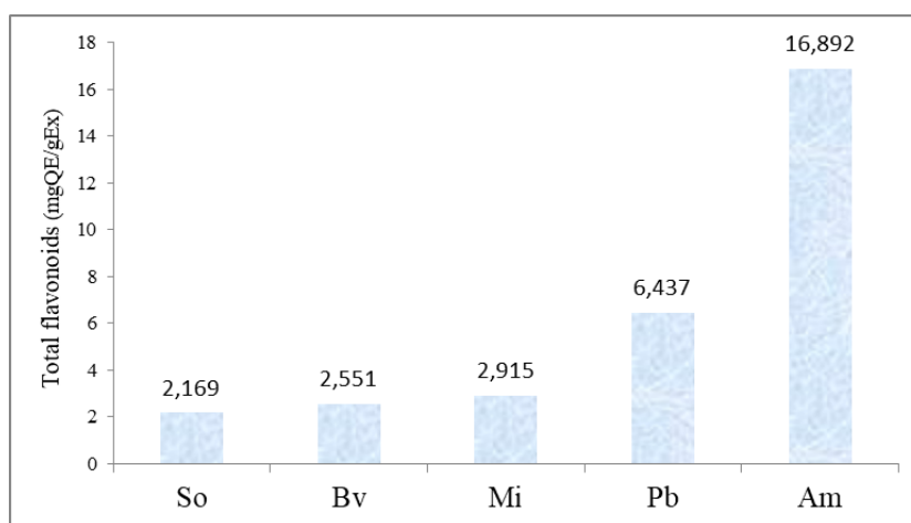
Fig. 3. Total flavonoids content of hydroethanolic plant extract
