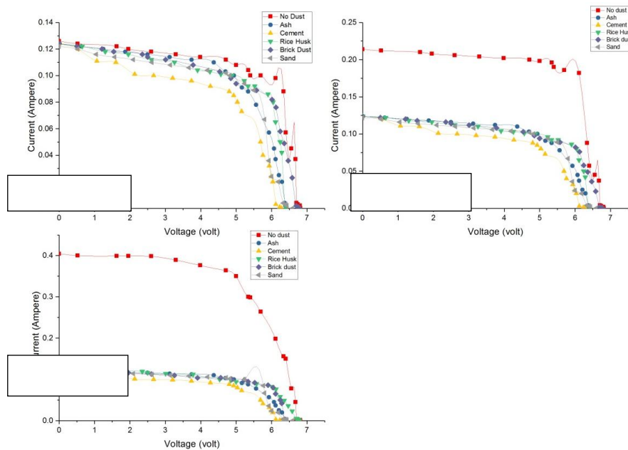
Fig. 3. I-V characteristics for three different solar irradiances
