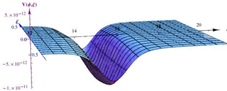
Fig. 2. The Ekpyrotic superpotential has been defined in terms of the potentials V(\phi, \xi) which is presented in the paper as V(\phi_0, \phi_1) where V(\phi_1) = 0 for b = \sqrt{3} , d = 1 that in essence shows the decreasing potential \phi_{ekpyrotic-end} with a negative gradient that falls steeply with a saddle-like curvature and bounces back with a non-locally flat curvature satisfying the FLRW [see Appendix B] metric with a small local positive curvature
