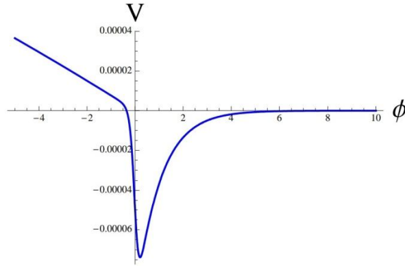
Fig. 1. Generic diagram of the Ekpyrotic Scalar Potential. Figure from [2]
